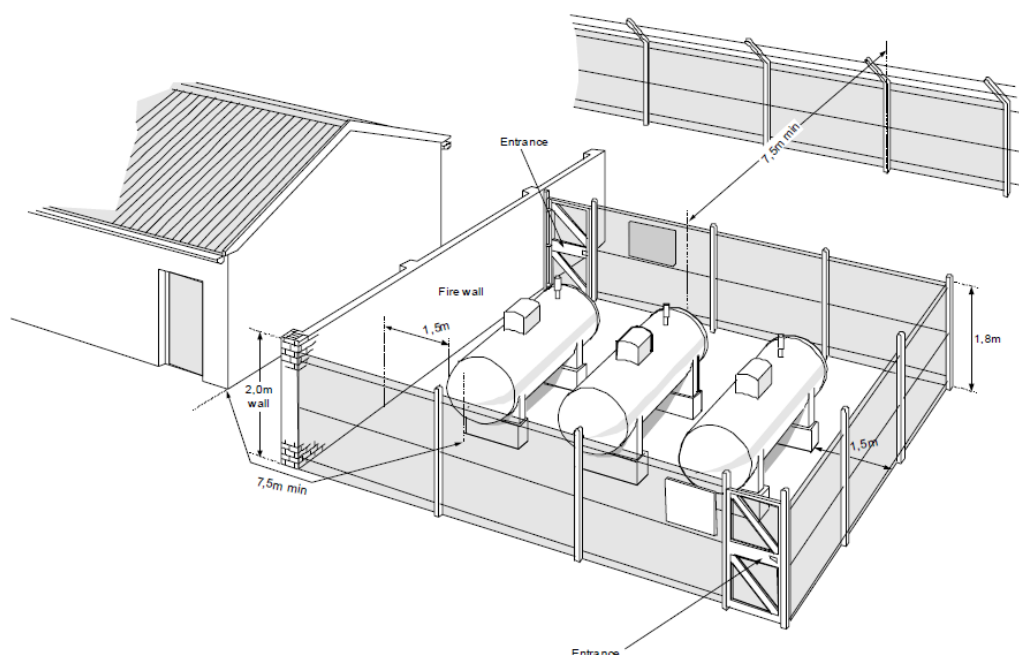
Figure 2 - Tank compound with fire wall and security fence (Source: UK LPGA COP 1)
