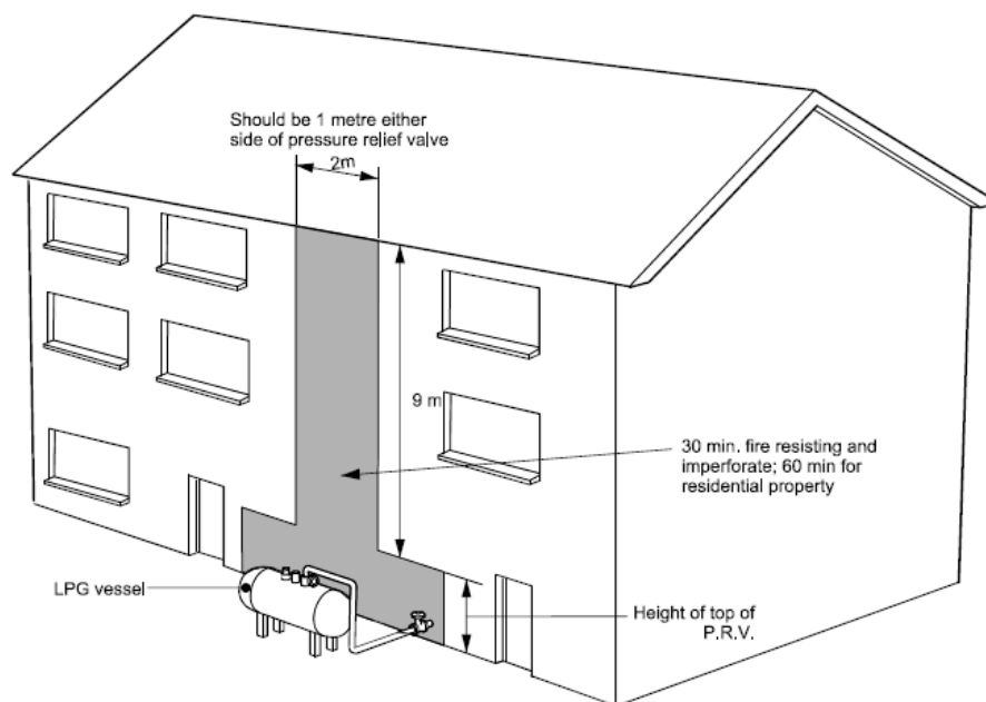
Figure 1 - Fire wall for tanks 2,500 litres or less (Source: UK LPGA COP 1)
